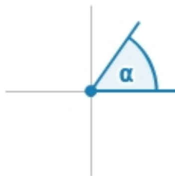
spitzer Winkel 0^\circ < \alpha < 90^\circ
